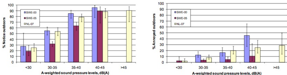
Left graph: % that can hear the turbines at each sound level Right graph: % that is “rather” or “very” annoyed at each sound level Maroon (center) bars are the suburban site; purple and yellow are the rural sites
